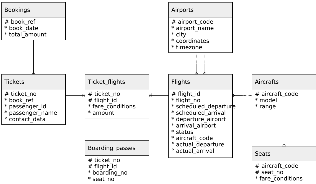
Figure M.2. Bookings Schema Diagram
