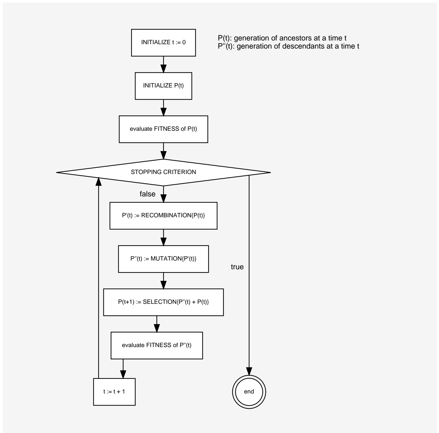
Figure 62.1. Structure of a Genetic Algorithm
