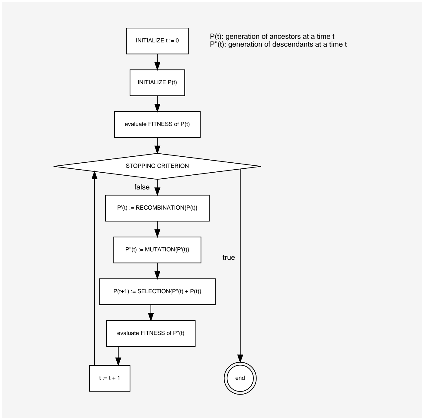
Figure 58.1. Structure of a Genetic Algorithm
