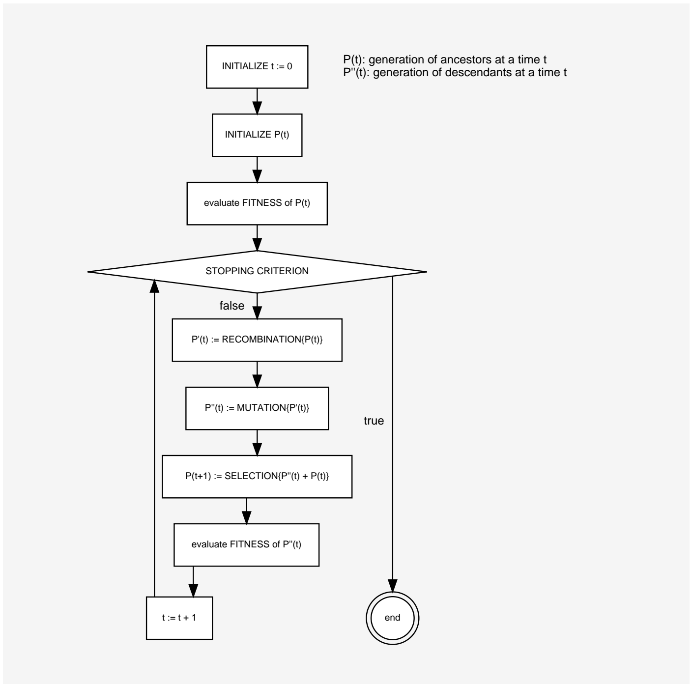
Figure 59.1. Structure of a Genetic Algorithm
